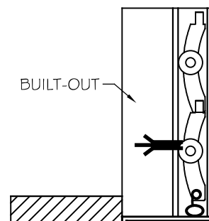
SECTION DD SILL WALL / BUILT-OUT SECTION
